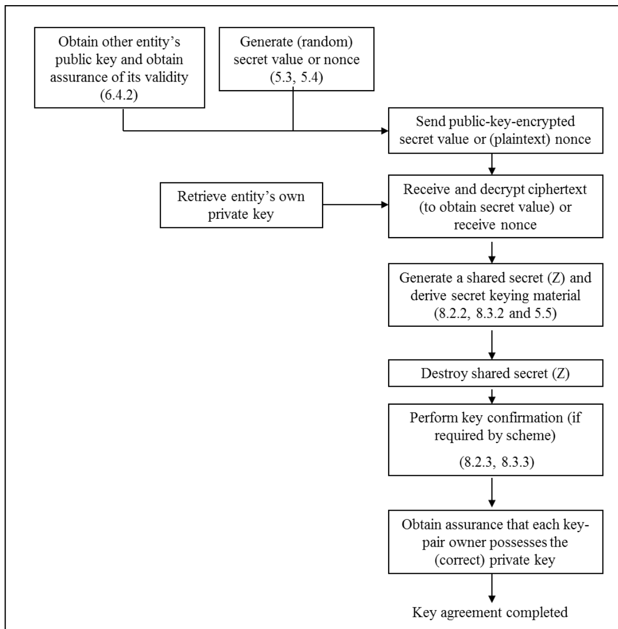
Figure 2: Key-Agreement Process
