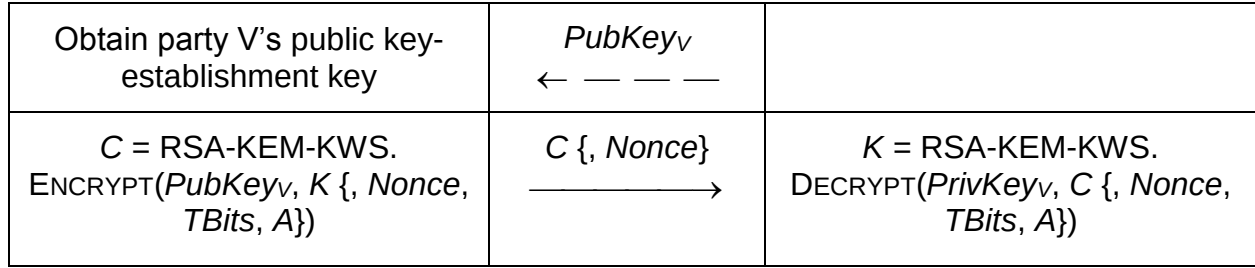
Figure 16: KTS-KEM-KWS-basic Scheme
