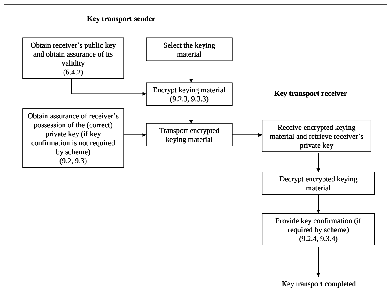
Figure 3: Key-transport Process
