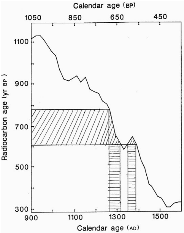
Fig. 17. Transformation of the Radiocarbon Age (BP) to the Calendar Age (AD) of the Shroud. The 14 C age (95 % CI) of (691 ± 31) BP corresponds to a two-valued calendar age as a result of the non-monotonic radiocarbon dating calibration curve. As indicated in the figure, the projected calendar age ranges are: (1262–1312) AD and (1353–1384) AD [38].
