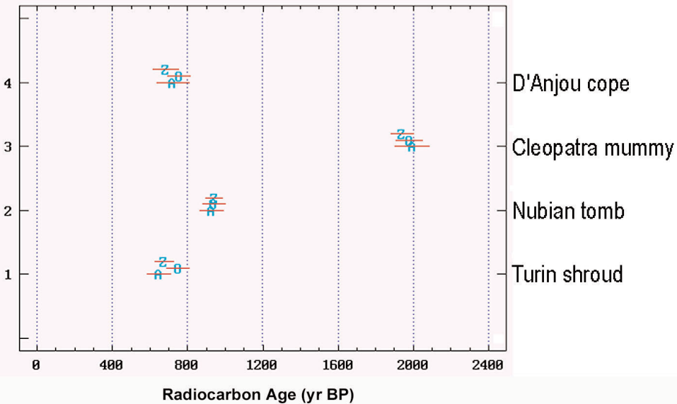
Fig. 16. AMS 14 C dating results (“blind”) for the Turin Shroud (sample-1) and three control samples of known age (samples-2,3,4), from the three AMS laboratories: Z (Zürich), O (Oxford), and A (Arizona). Dates are expressed as “Radiocarbon Years” before present (BP); uncertainties represent 95 % confidence intervals [38].
