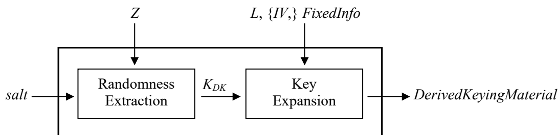
Figure 1: The Extraction-then-Expansion Key-Derivation Procedure
