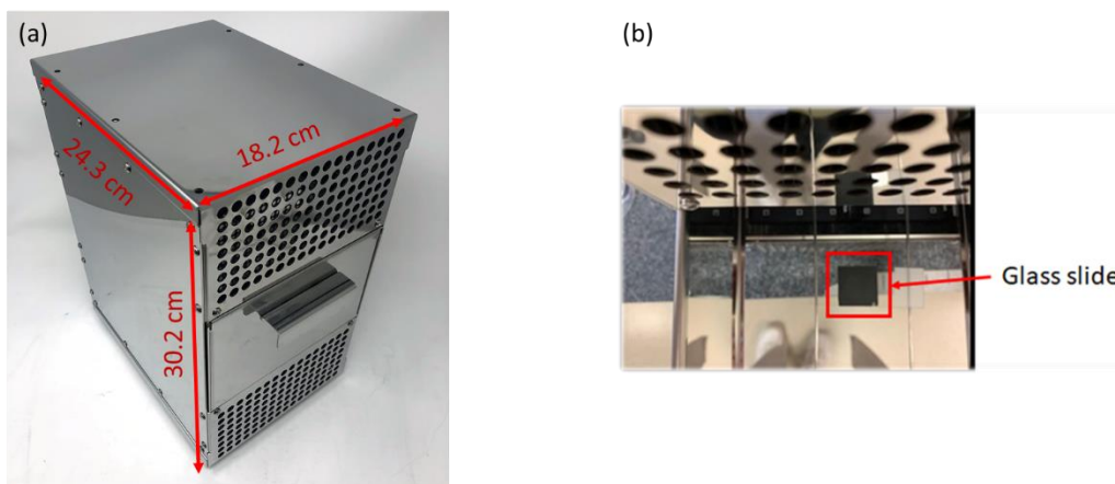
Fig. 15. (a) Photograph of the prototype device and (b) glass slide placed inside the tray.
