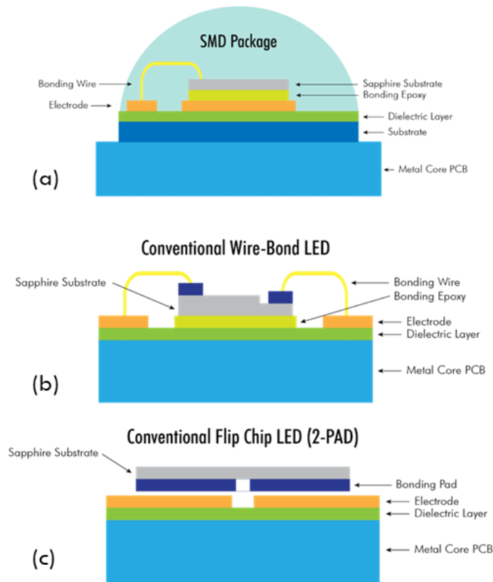
Fig. 7. Different packaging technologies used in manufacturing commercial UV-LEDs: (a) surface mount devices (SMDs), (b) conventional wire-bond technology, and (c) standard flip-chip technology (two-pad technology). PCB is printed circuit board.
