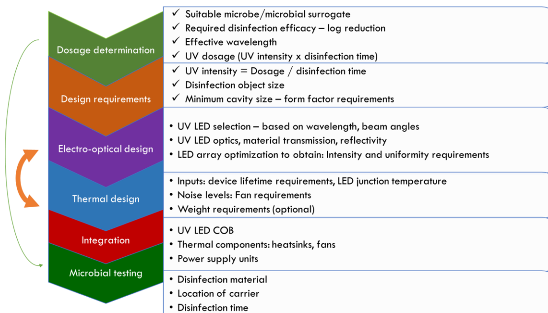
Fig. 16. Summary of the overall design process for a surface disinfection device.
