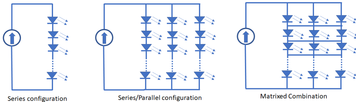
Fig. 5. Different LED array formats define the voltage-current requirements for the PSU. LEDs may be connected in series or parallel configuration or in a matrixed combination in a chip-on-board format.
