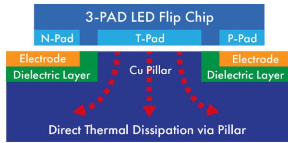
Fig. 8. Structure of a three-pad UV-LED with a thermal pad and a copper pillar that direct the heat away from the LED.
