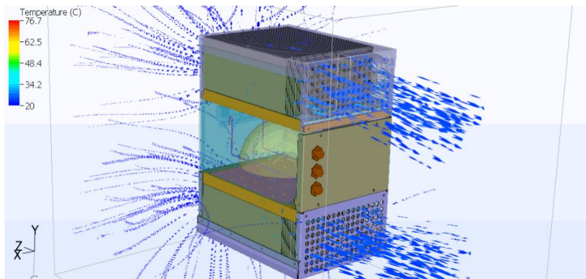
Fig. 13. Thermal simulations performed with heat sinks and fans for the surface disinfection device.
