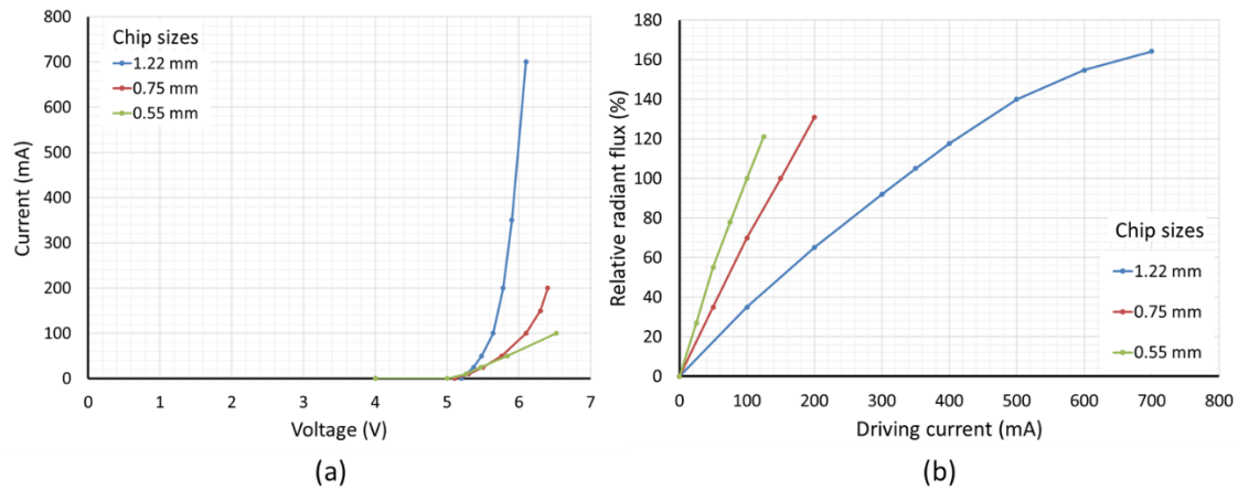
Fig. 3. (a) Current-voltage curve for three chip sizes of a 265 nm UV-LED. (b) Relative radiant flux as a function of drive current for three chip sizes of a 265 nm UV-LED. The relative radiant flux values are taken at the typical driving current for each chip size, adapted from Ref. [23].
