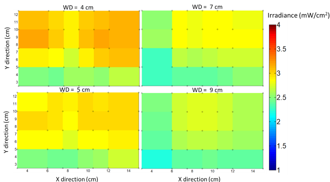
Fig. 14. UV irradiance data measured at different working distances with only the top UV-LED array turned ON.
