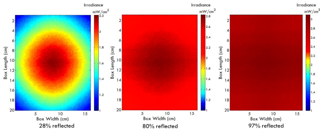
Fig. 12. Variation in irradiance profiles with varying degree of side-wall reflections.
