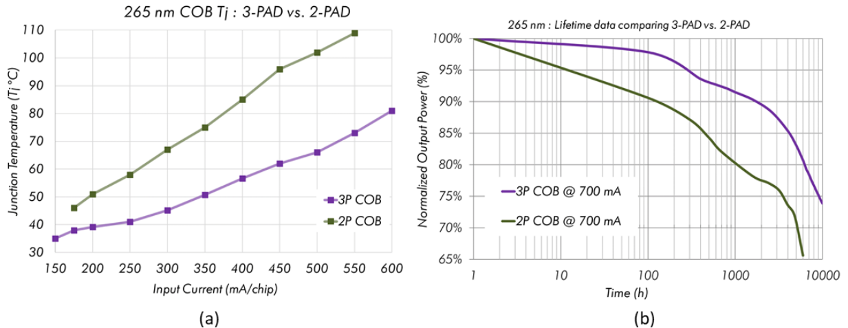
Fig. 9. Experimental results comparing the two-pad and the three-pad technology, showing (a) the junction temperature as a function of driving current and (b) the normalized optical output as it degrades with time.
