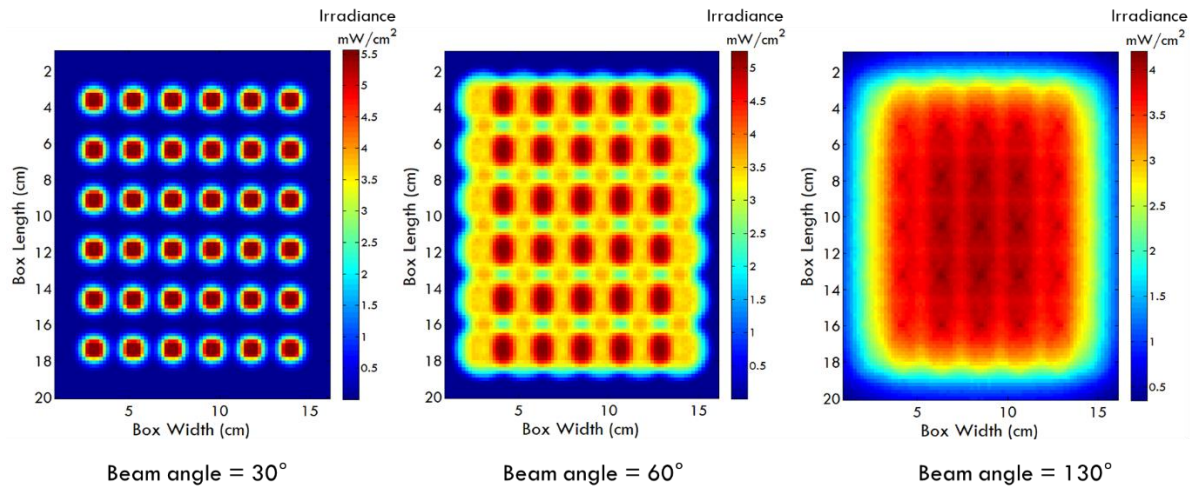
Fig. 4. Variation in irradiance distributions with varying UV-LED beam angles. Irradiance hot spots are predominant with lower beam angles and lower working distances.
