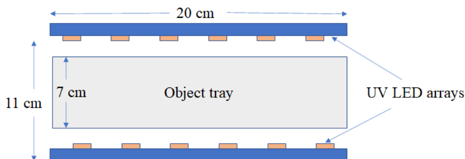
Fig. 11. Cross section and dimensions of the UV-LED chamber.
